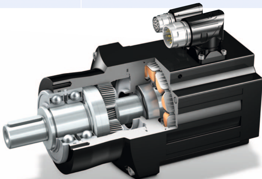
Section: SMS PE_EZ planetary geared motor
