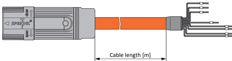
Fig. 2: Length definition for ready-made power cables – SB6, SC6, S16
