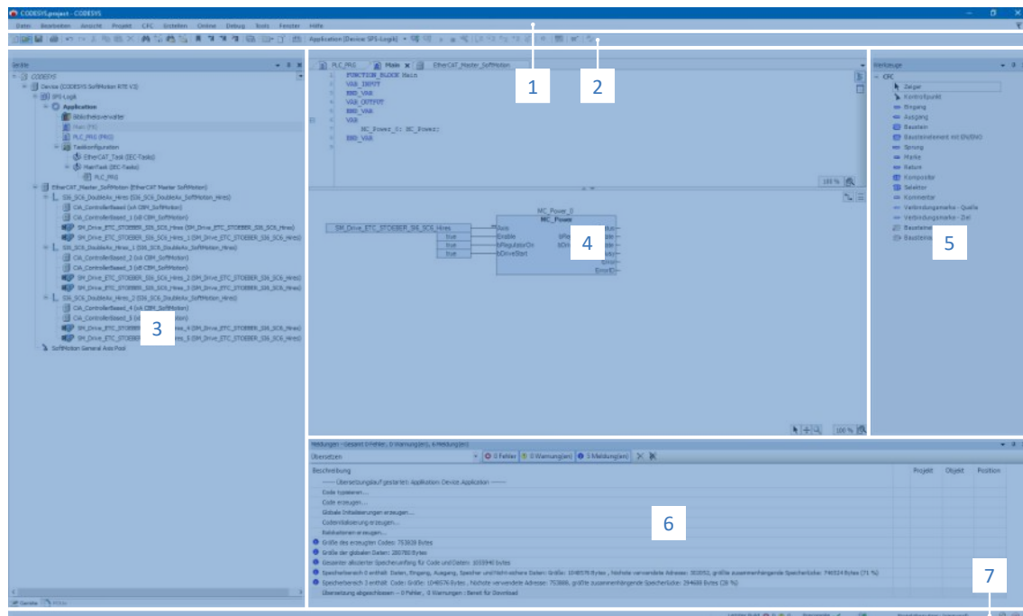
Fig. 4: CODESYS Development System V3 : interface programme
