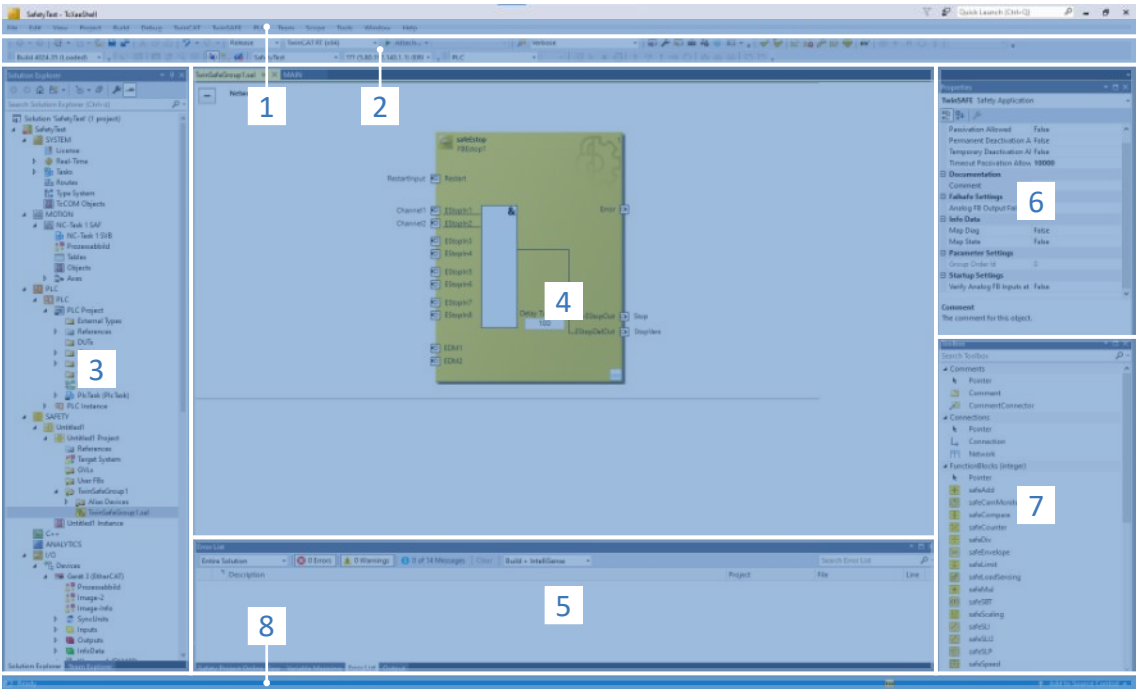
Fig. 3: TwinCAT 3 Engineering : Interface programme
