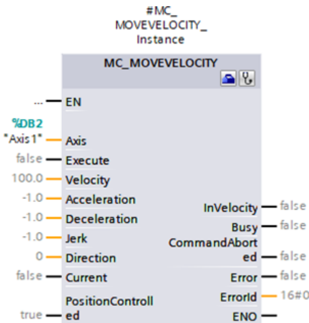
Abb. 8: PLCopen-Baustein MC_MOVEVELOCITY
