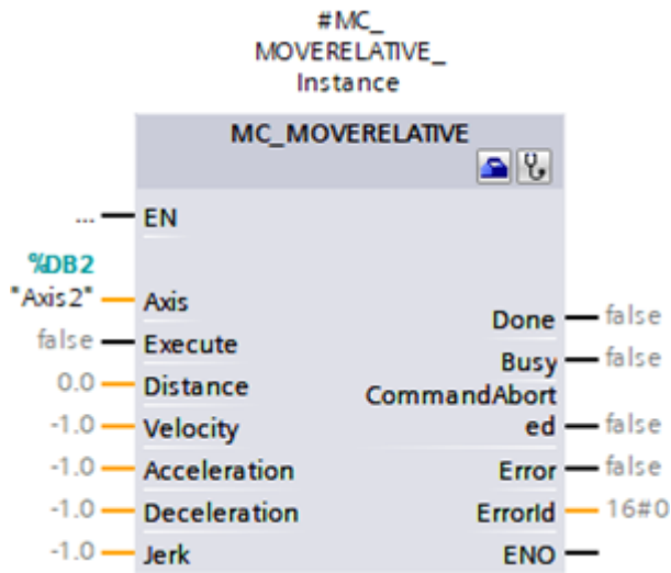
Abb. 18: PLCopen-Baustein MC_MOVERELATIVE
