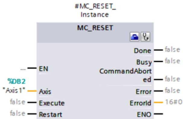
Abb. 16: PLCopen-Baustein MC_RESET
