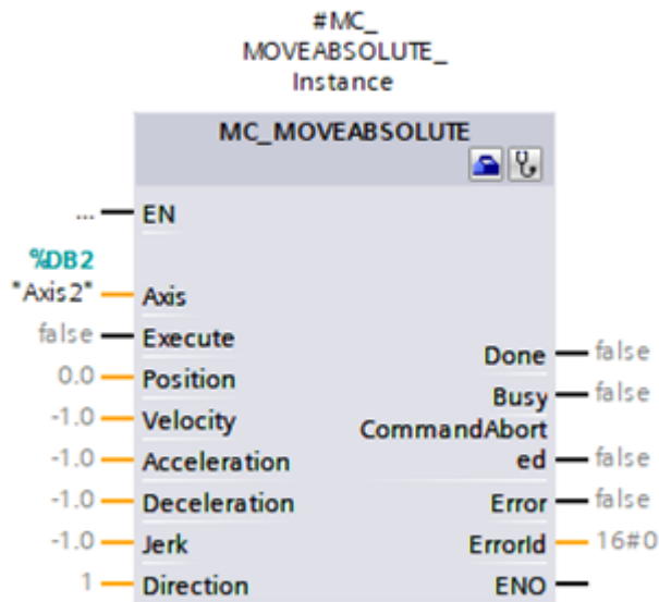
Abb. 19: PLCopen-Baustein MC_MOVEABSOLUTE
