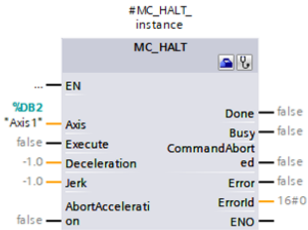
Abb. 15: PLCopen-Baustein MC_HALT
