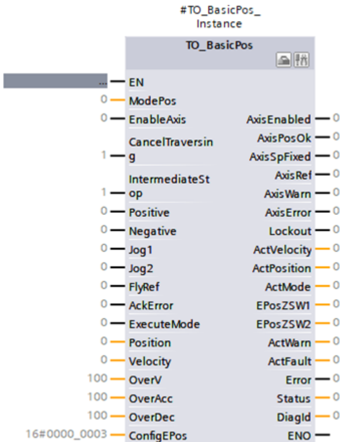
Abb. 23: Baustein TO_BasicPos
