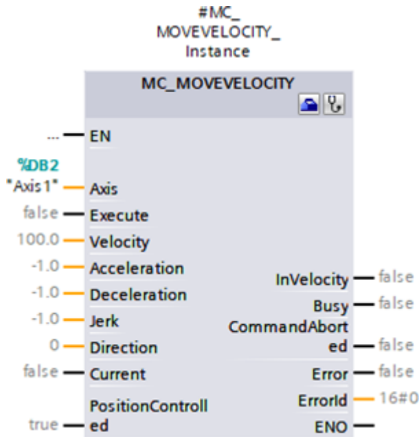
Abb. 13: PLCopen-Baustein MC_MOVEVELOCITY
