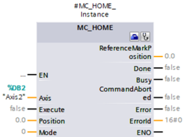
Abb. 17: PLCopen-Baustein MC_HOME
