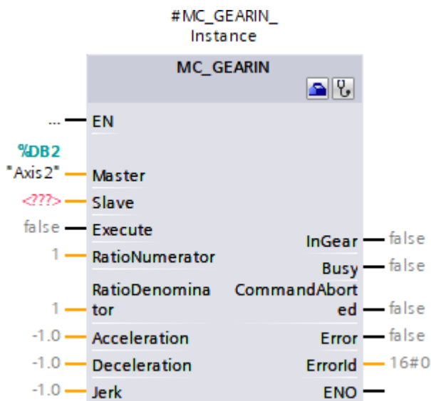
Abb. 21: PLCopen-Baustein MC_GEARIN
