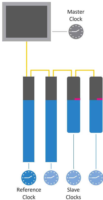
Abb. 12: EtherCAT: Distributed Clocks
