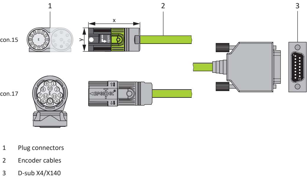
Encoder cables – con.15 plug connectors
