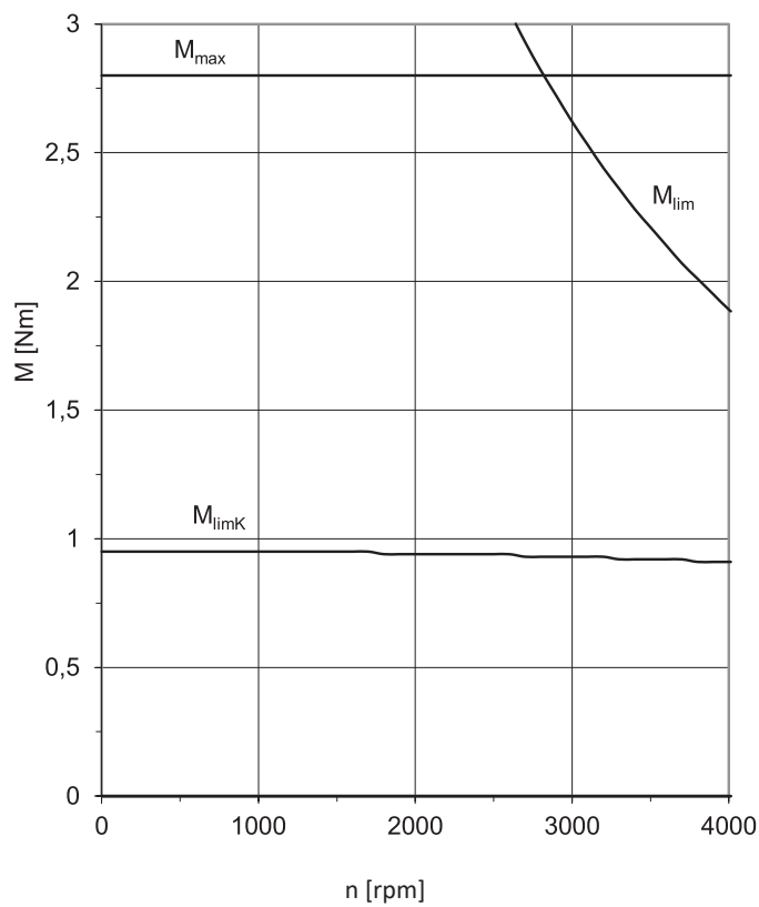
EZ301 ( n_N=3000 rpm)
