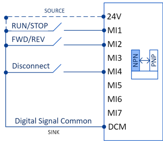
Figure 3: cLEAN Input Wiring Example
