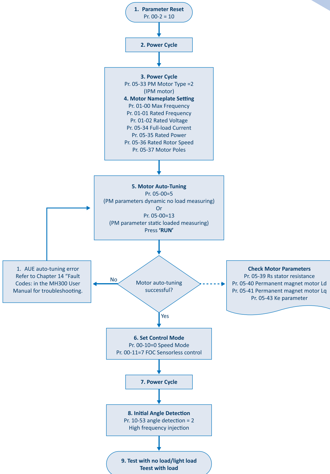
Figure 2: IPM Sensorless Adjustment Flowchart
