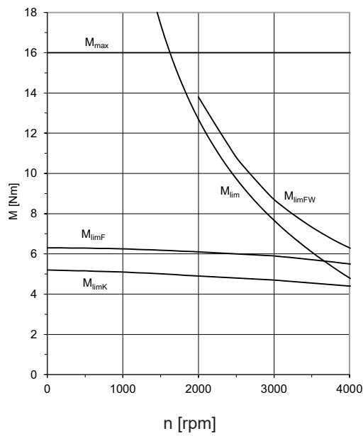
EZ402 ( n_N=3000 rpm)
