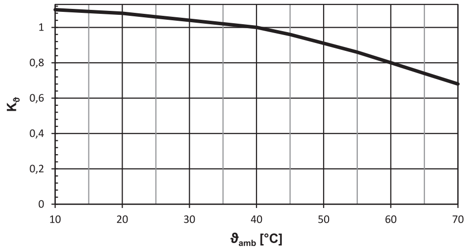
Fig. 7: Derating depending on the surrounding temperature
