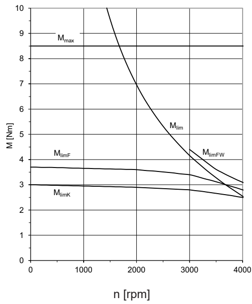
EZ401 ( n_N=3000 rpm)
