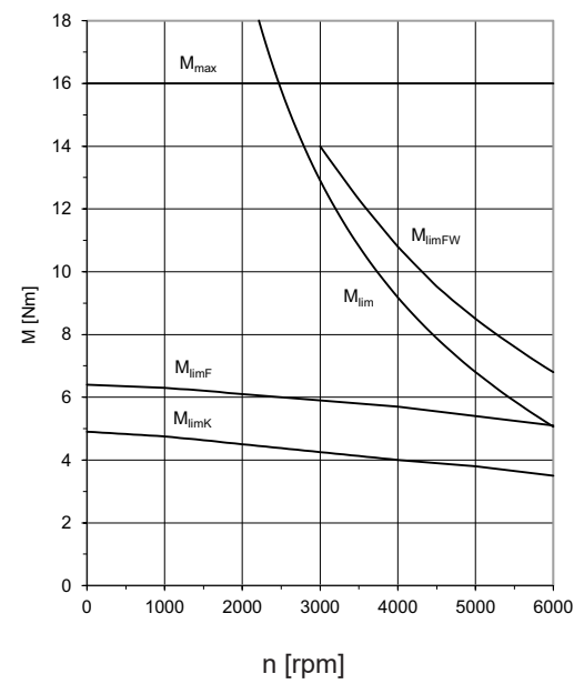
EZ402 ( n_N=6000 rpm)
