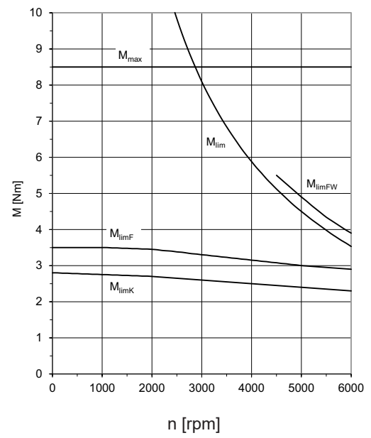
EZ401 ( n_N=6000 rpm)
