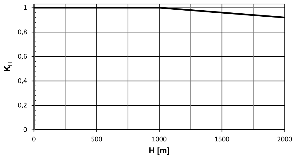
Fig. 8: Derating depending on the installation height
