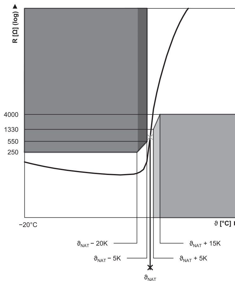
Fig. 6: PTC thermistor curve (single thermistor)
