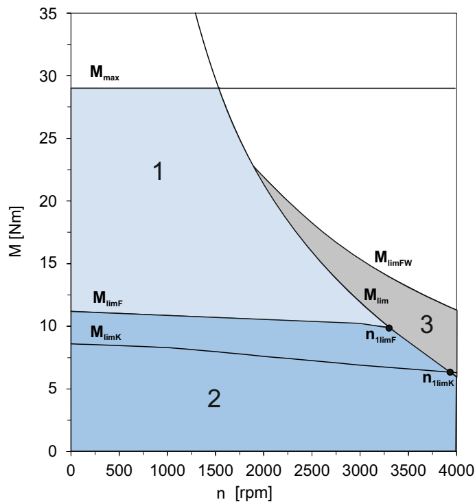
Fig. 9: Explanation of a torque/speed curve
