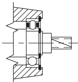
Backstop for all units using: MRB140/050, MRB160/050, MRB160/140
