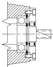
Backstop for MRB200/050 through MRB200/180.
