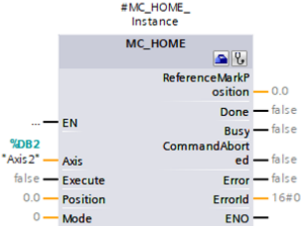
Abb. 17: PLCopen-Baustein MC_HOME
