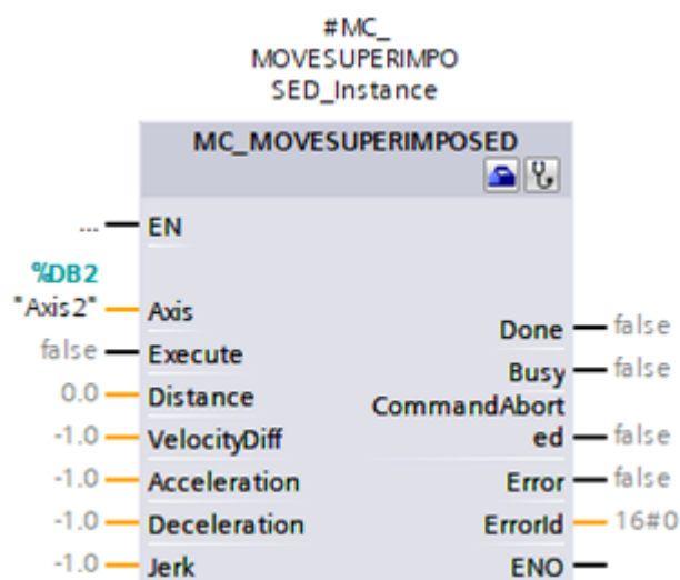
Abb. 22: PLCopen-Baustein MC_MOVESUPERIMPOSED
