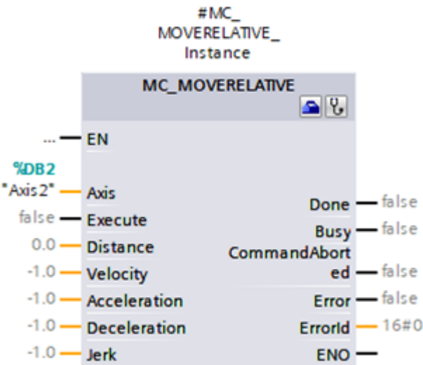
Abb. 18: PLCopen-Baustein MC_MOVERELATIVE
