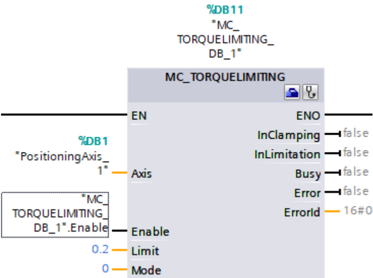
Abb. 10: PLCopen-Baustein MC_TORQUELIMITING
