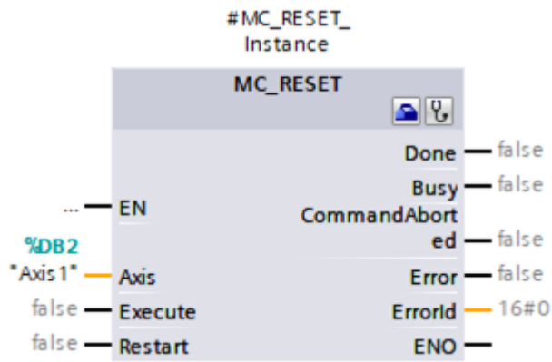
Abb. 7: PLCopen-Baustein MC_RESET
