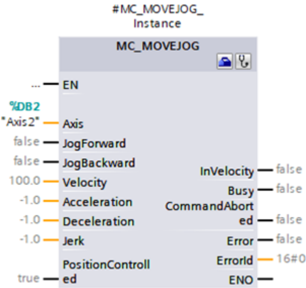
Abb. 20: PLCopen-Baustein MC_MOVEJOG
